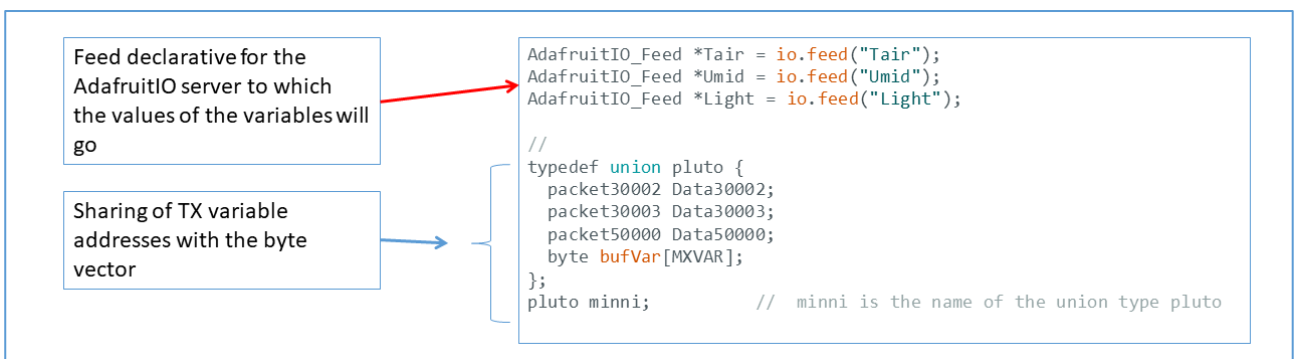
Figure 18 - Packet.h content, second part
