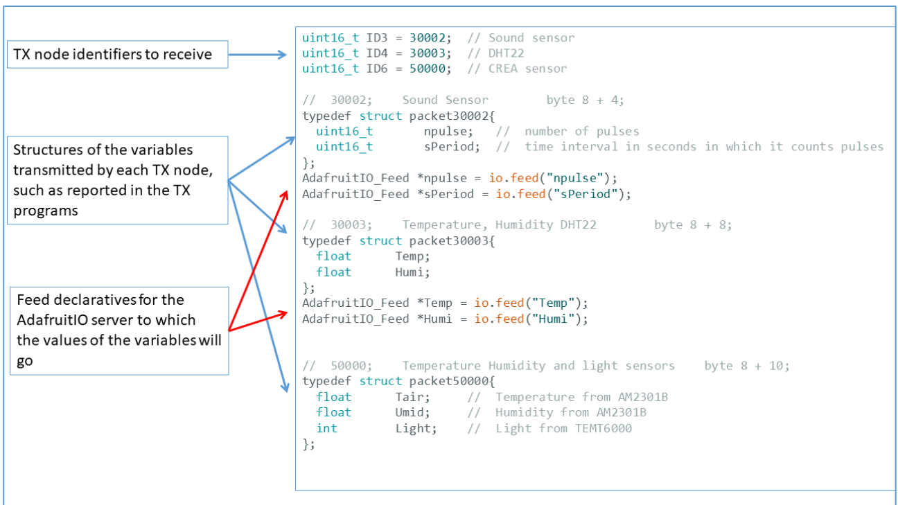
Figure 17 - Packet.h content, first part
